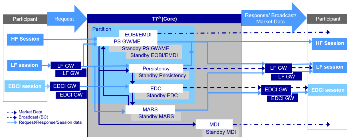
Fig. 3-1: Schematic overview of T7 components and data streams
