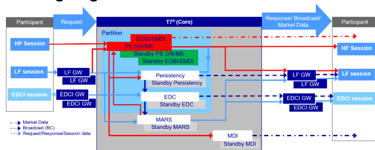
Fig. 3-5: PS Gateway/Matching Engine failover
