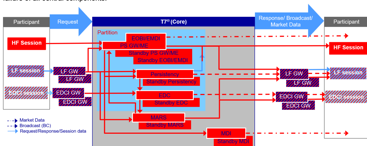
Fig. 3-10: Failure and restart of the complete T7 system
