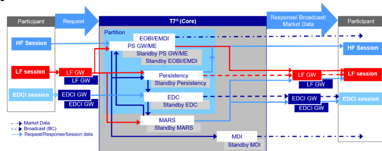
Fig. 3-2: LF Gateway failure
